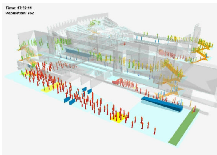
Figure 14: MassMotion Theatre Model
