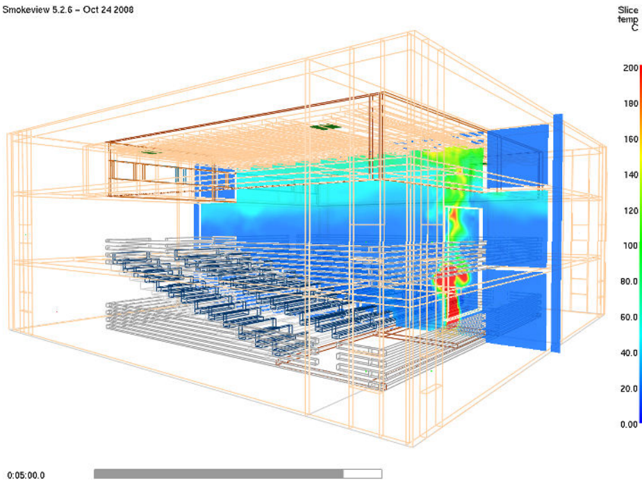
Figure 4: Smoke Modelling of the Auditorium
