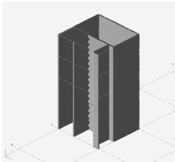
Fig. 9 Concrete core (shear wall) elements in GSA (isometric view)
