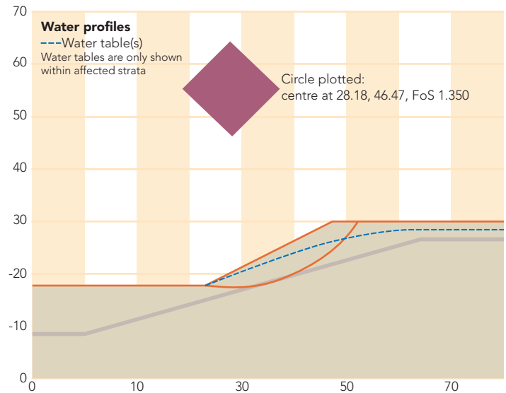
FIGURE 11: LOWEST FOS CIRCULAR SLIP SURFACE ASSUMING SLIP FORMS TANGENT TO BASE OF LOW STRENGTH STRATA
