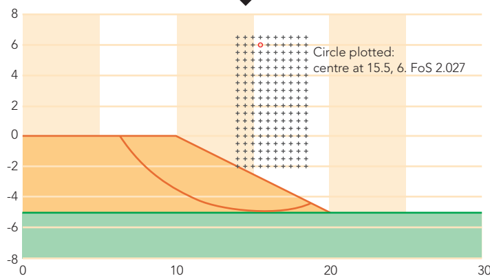
FIGURE 4: EXAMPLE C SLOPE RESULT – FAILURE SURFACE PRESUMED TO BE TANGENT TO STRATUM 2
