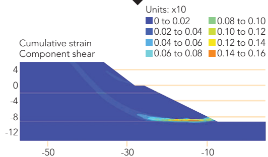
FIGURE 8: CRITICAL SLIP SURFACES LOCATED USING FE MODELLING. (Note presence of second smaller slip surface in upper layer)
