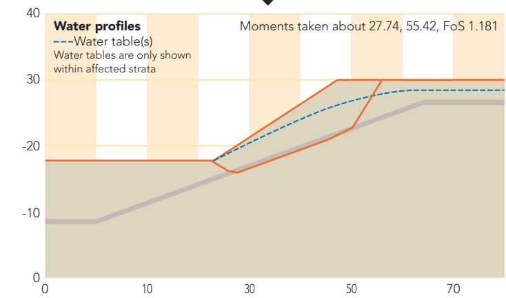
FIGURE 14: RESULTS FOR THE NON-CIRCULAR LE SLOPE MODEL WITH SLIP GEOMETRY DERIVED FROM FE MODELLING
