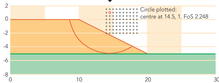
FIGURE 3: EXAMPLE C SLOPE RESULT – INITIAL ATTEMPT TO IDENTIFY CRITICAL SLIP SURFACE BY VARYING SLIP CIRCLE CENTRE AND RADII
