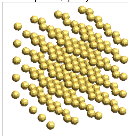
Spheres, quality = 2
