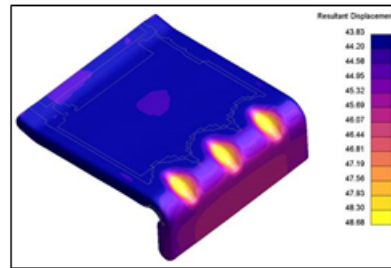
Plasma
