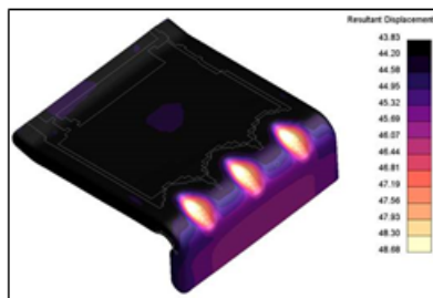
Magma
