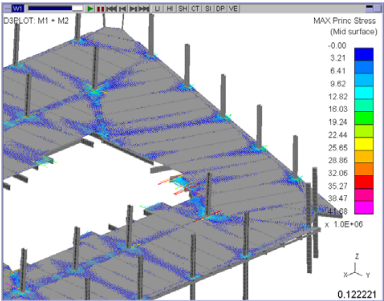
PR plot only show Max Principal Stress
